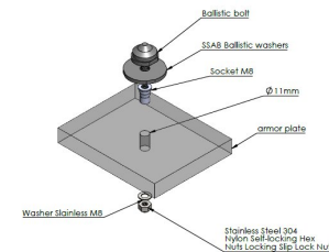
Figure 1. Exploded system assembly.
